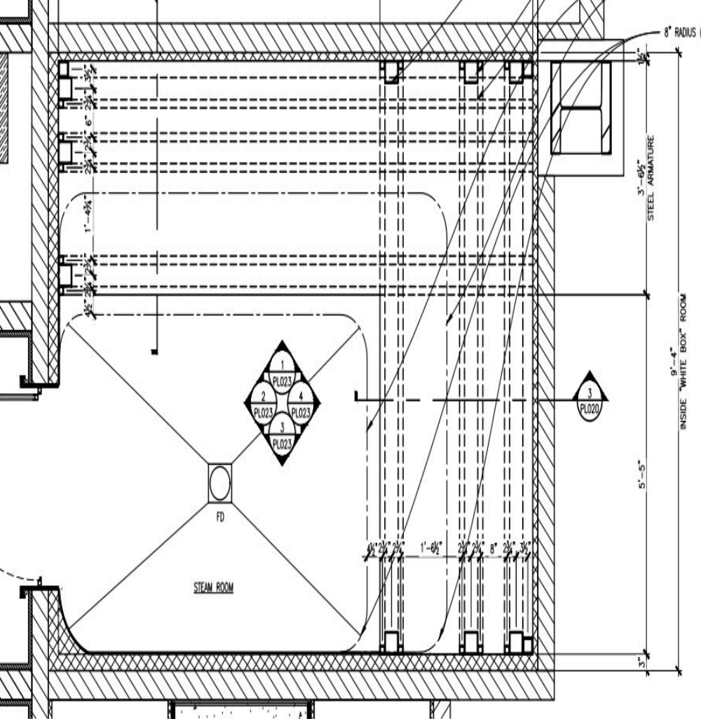
5 STEAM ROOM FRAMING PLAN
